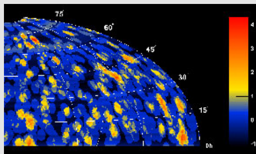
Sky map from the AMANDA neutrino telescope. Image courtesy of Andrea Silvestri, AMANDA, UCI
